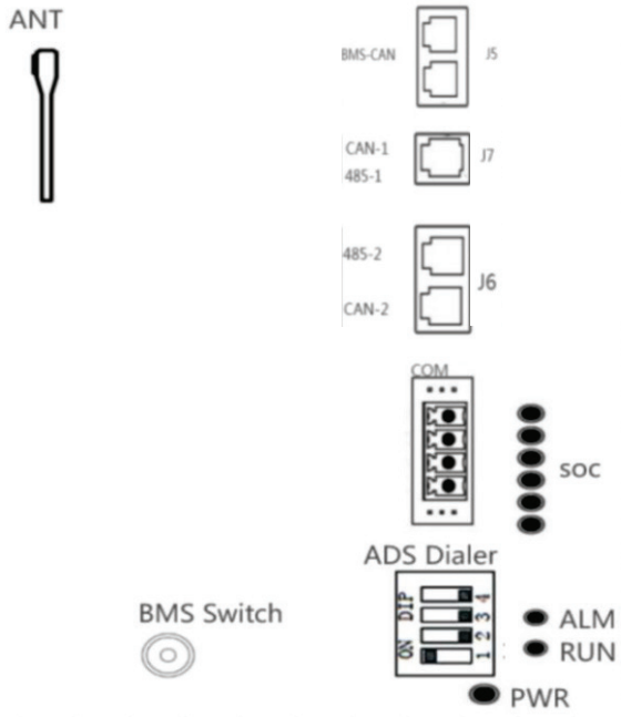
Fig. 5-2 Peration Panel
