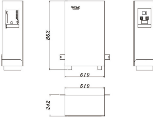
Fig. 5-1 Product Dimensions
